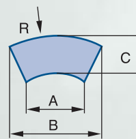
Shape 3104 - B x A x R x L
